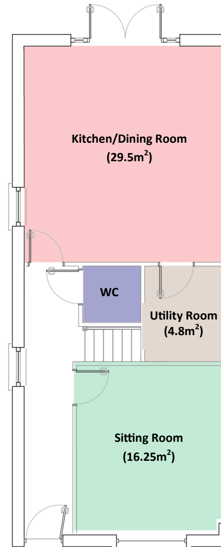
GROUND FLOOR
