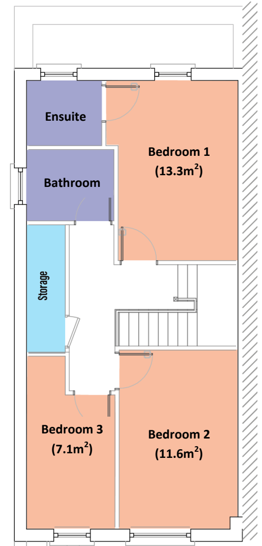
FIRST FLOOR
